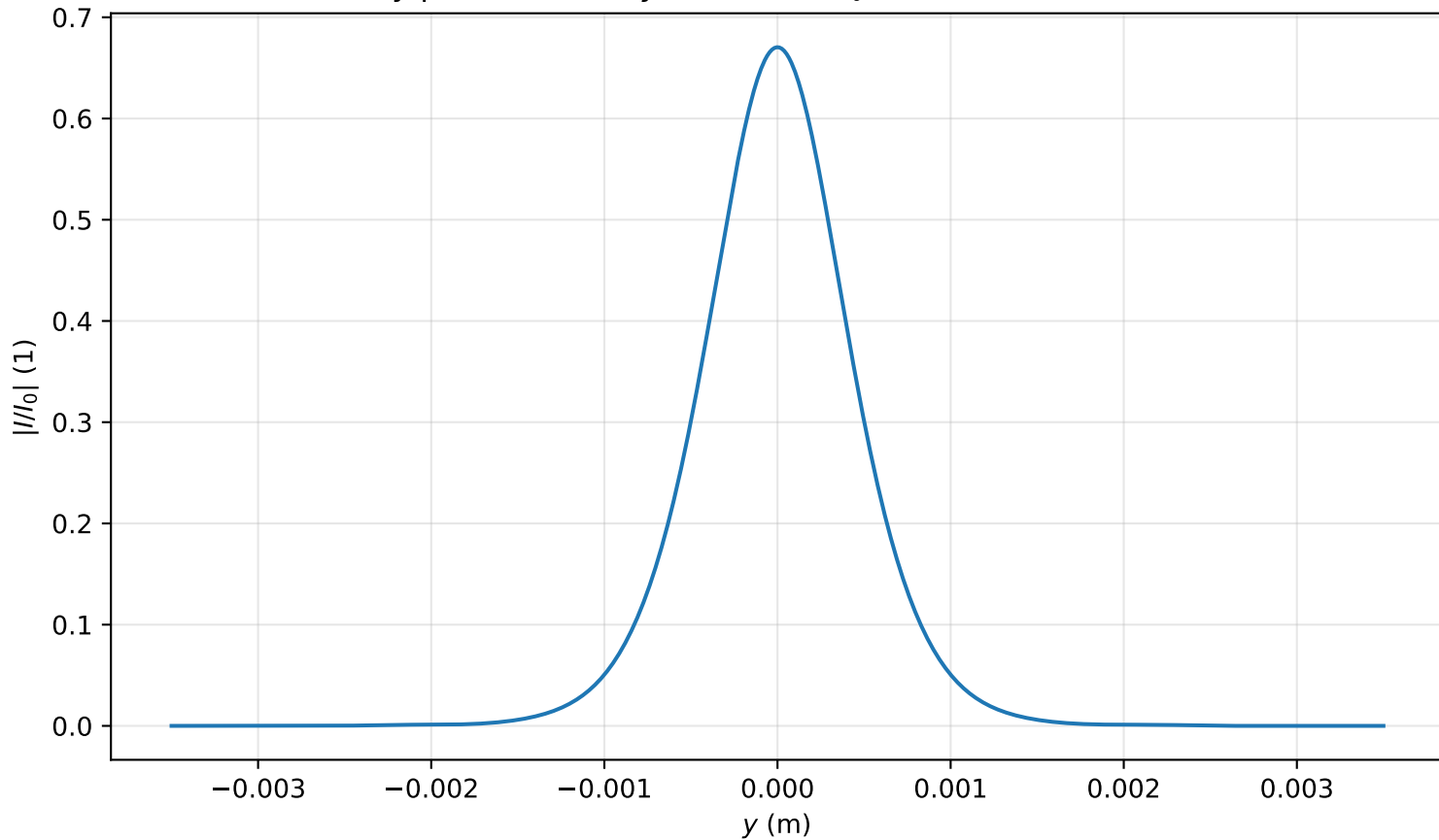
Intensity profile I(x=0, y, z=3.742)/I_0 , P_{in}=0.7P_{cr} , artificial time
